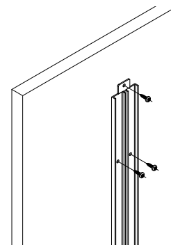
3 - Fixation M19 et cabochon. Fixing of channel & end cap
